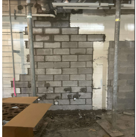
Continue to install CMU block infill around all in wall plumbing in area 2
